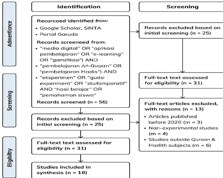
Gambar 1. PRISMA
