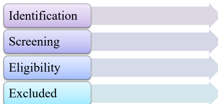
Diagram PRISMA
